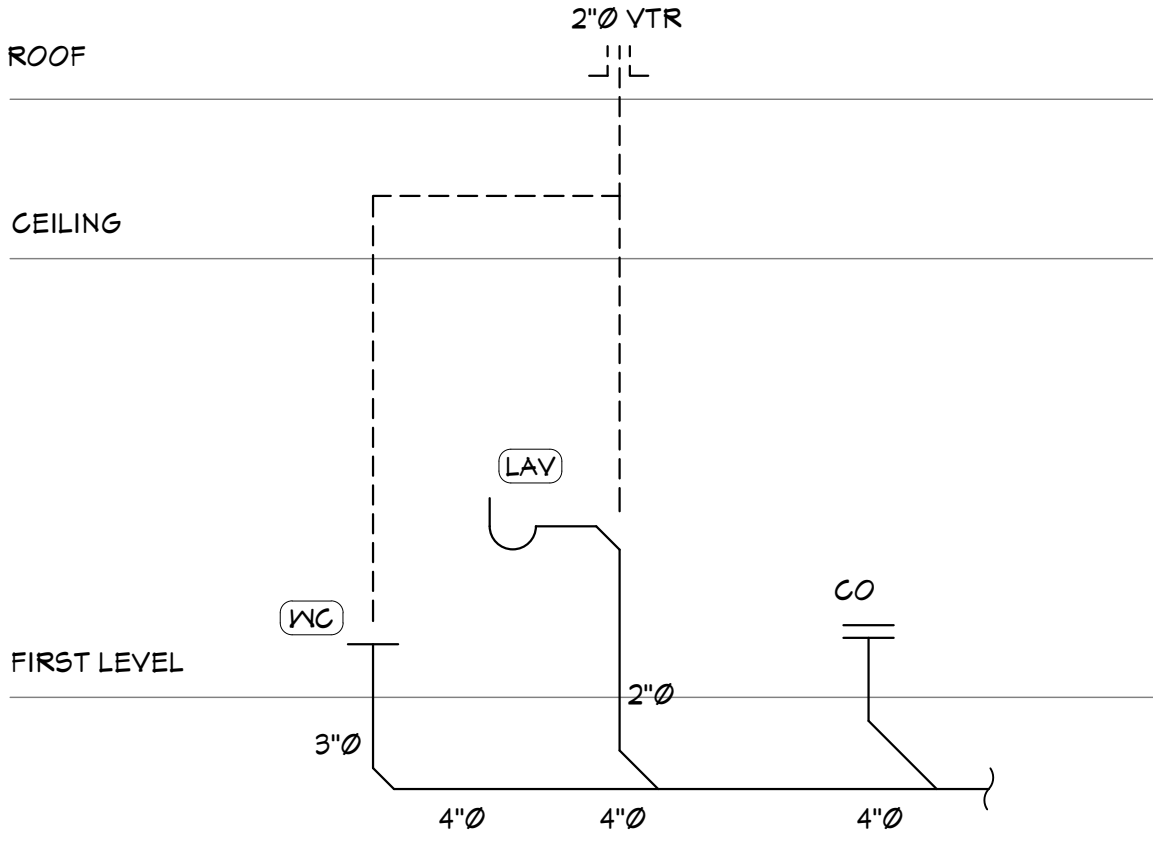
PLUMBING SANITARY RISER NTS
