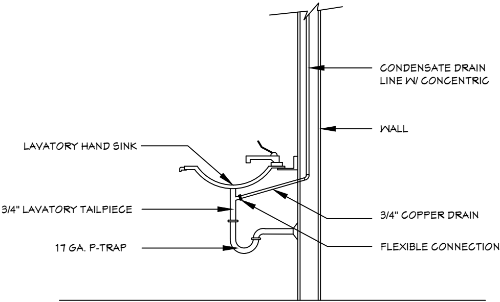
CONDENSATE DETAIL NO SCALE
