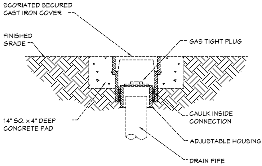
CLEANOUT TO GRADE SCALE:NONE
