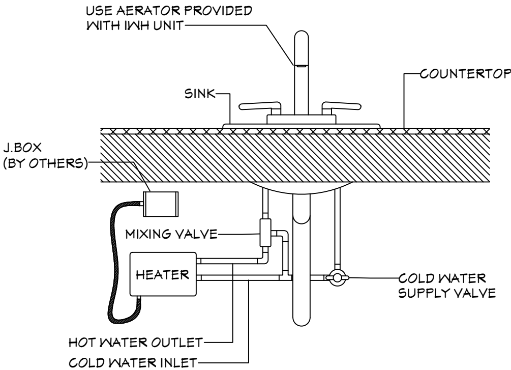
INSTA-HOT WATER HEATER DETAIL SCALE:NONE
